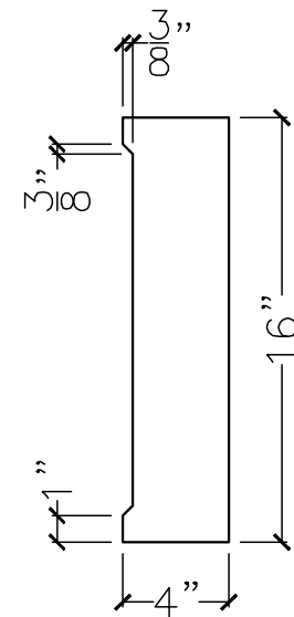
SECTION VIEW
