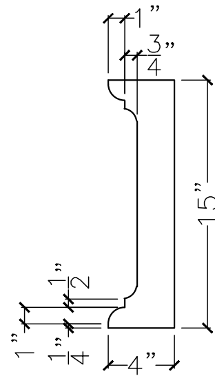
SECTION VIEW
