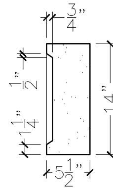
SECTION VIEW
