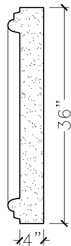
SECTION VIEW
