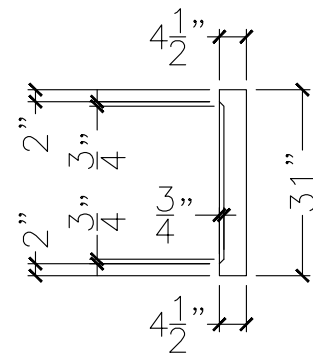
SECTION VIEW
