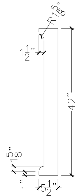
SECTION VIEW
