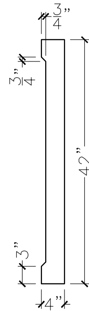
SECTION VIEW
