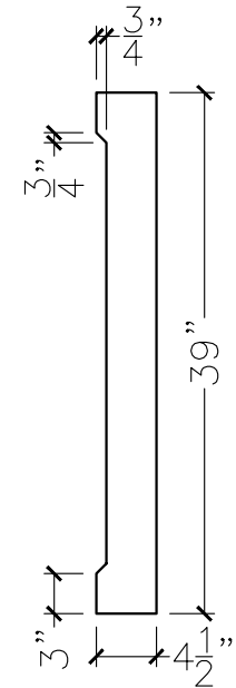
SECTION VIEW
