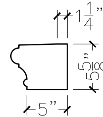
SECTION VIEW
