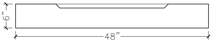
FRONT VIEW
