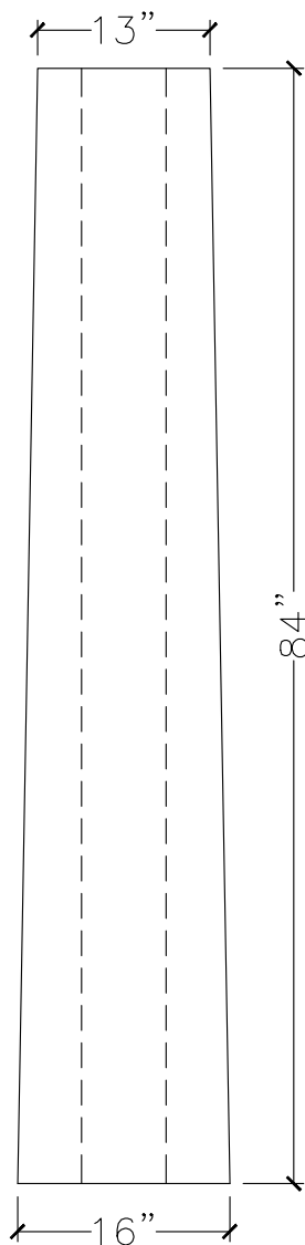
FRONT VIEW
