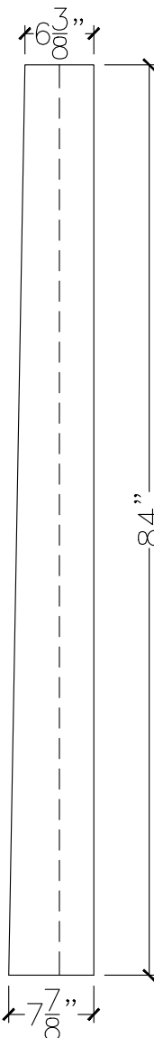
END VIEW
