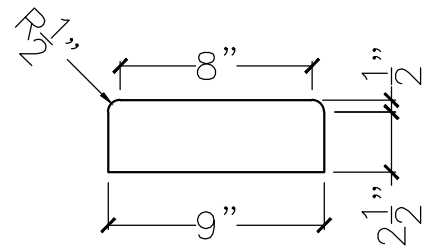
SECTION VIEW
