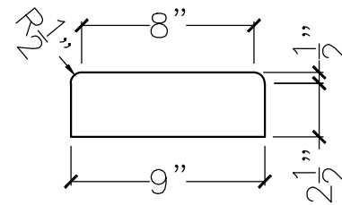
SECTION VIEW
