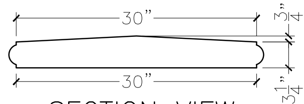
SECTION VIEW
