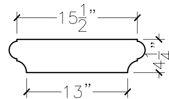
SECTION VIEW
