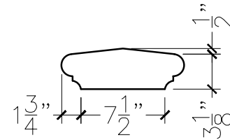
SECTION VIEW
