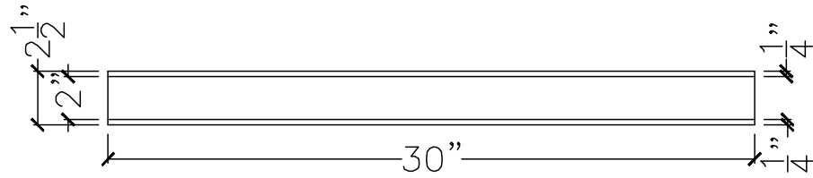
FRONT VIEW
