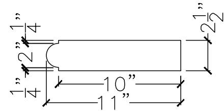
SECTION VIEW
