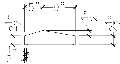
SECTION VIEW
