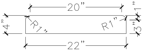
SECTION VIEW
