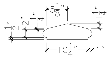
SECTION VIEW
