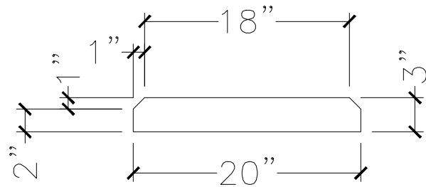
SECTION VIEW
