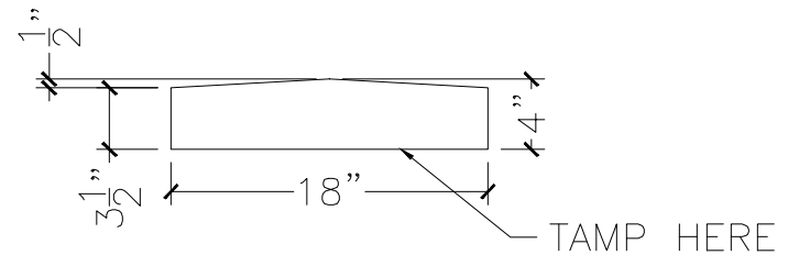
SECTION VIEW
