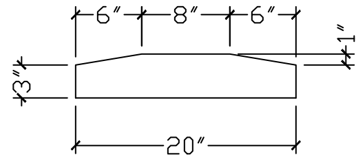
SECTION VIEW
