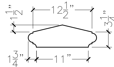
SECTION VIEW
