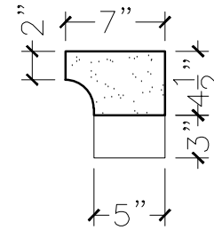
SECTION VIEW
