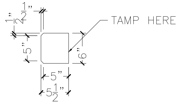
SECTION VIEW
