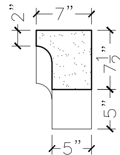
SECTION VIEW
