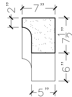
SECTION VIEW
