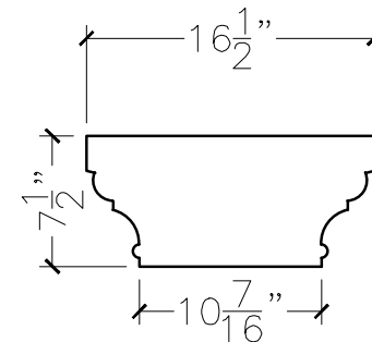
SECTION VIEW
