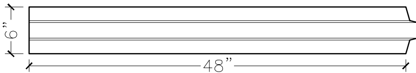
FRONT VIEW
