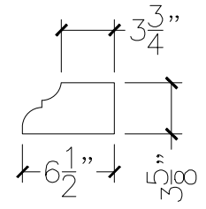
SECTION VIEW
