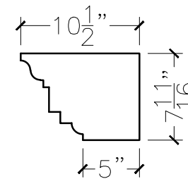
SECTION VIEW
