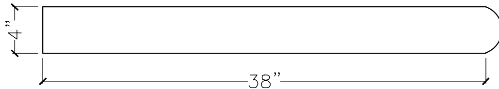
FRONT VIEW
