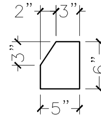
SECTION VIEW
