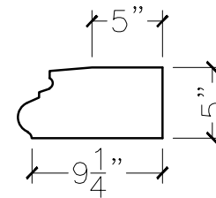
SECTION VIEW
