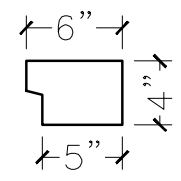
SECTION VIEW
