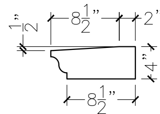
SECTION VIEW
