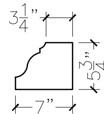
SECTION VIEW
