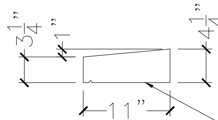
SECTION VIEW
