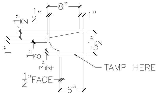
SECTION VIEW
