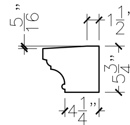
SECTION VIEW
