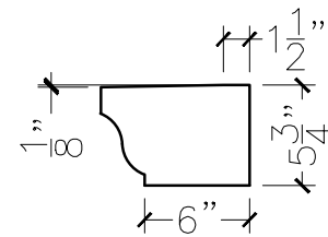
SECTION VIEW
