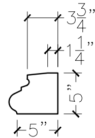
SECTION VIEW
