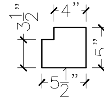
SECTION VIEW
