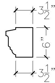
SECTION VIEW
