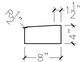
SECTION VIEW
