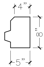
SECTION VIEW
