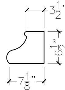
SECTION VIEW
