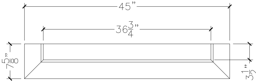
TOP VIEW
