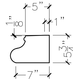
SECTION VIEW
