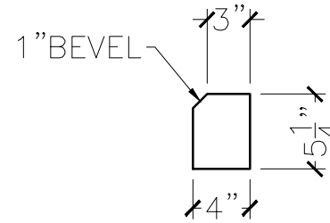
SECTION VIEW
